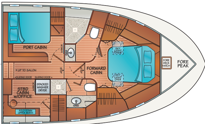
F55' – 3 CABIN 2 HEAD ACCOMMODATION w/VIP PORT + STBD OFFICE
