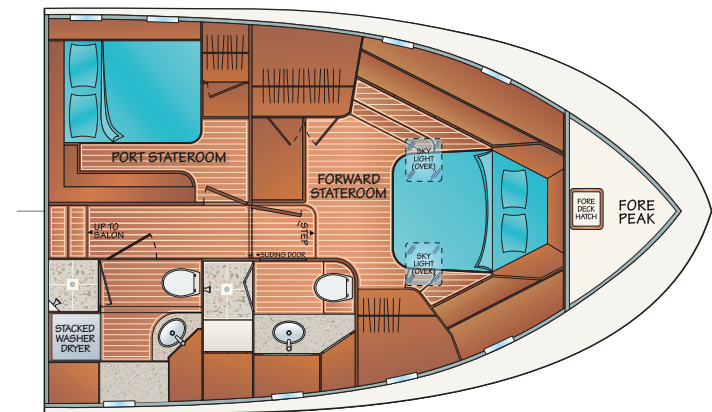
F55' – 2 STATEROOM 2 HEAD ACCOMMODATION
