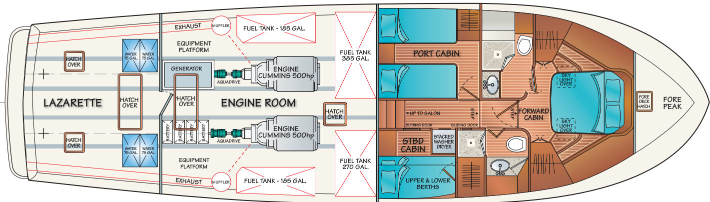
FLEMING 55' – LAZARETTE | ENGINE ROOM and STANDARD ACCOMMODATION (SHOWN w/STANDARD CUMMINS QSC 500HP ENGINES)
