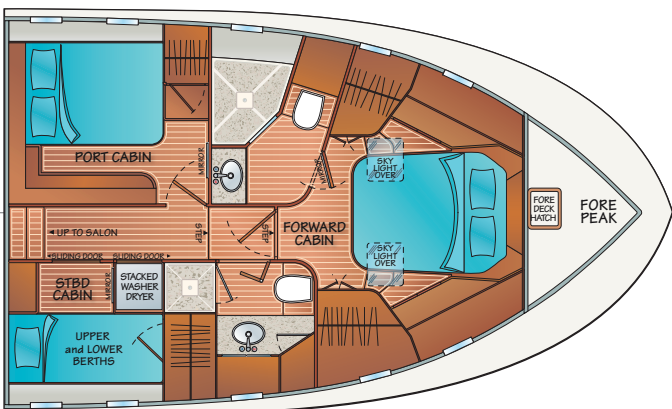
F55' – 3 CABIN 2 HEAD ACCOMMODATION –w/VIP PORT
