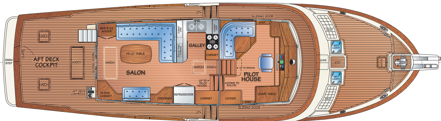
FLEMING 55' – MAIN DECK – SALON OPTION w/STBD SETTEE | PILOTHOUSE
