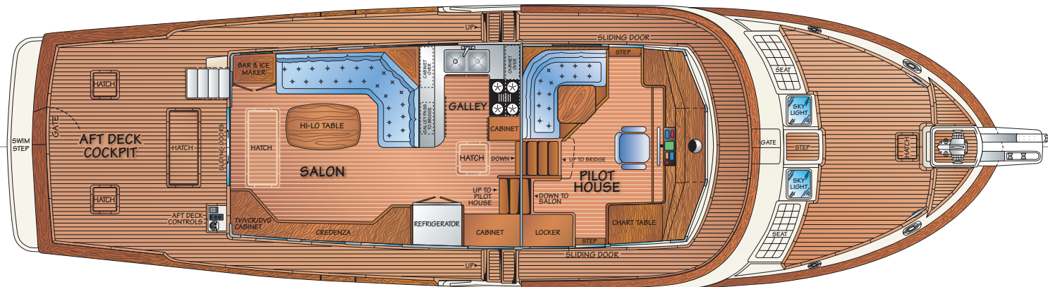
FLEMING 55' – MAIN DECK – SALON & PILOTHOUSE
