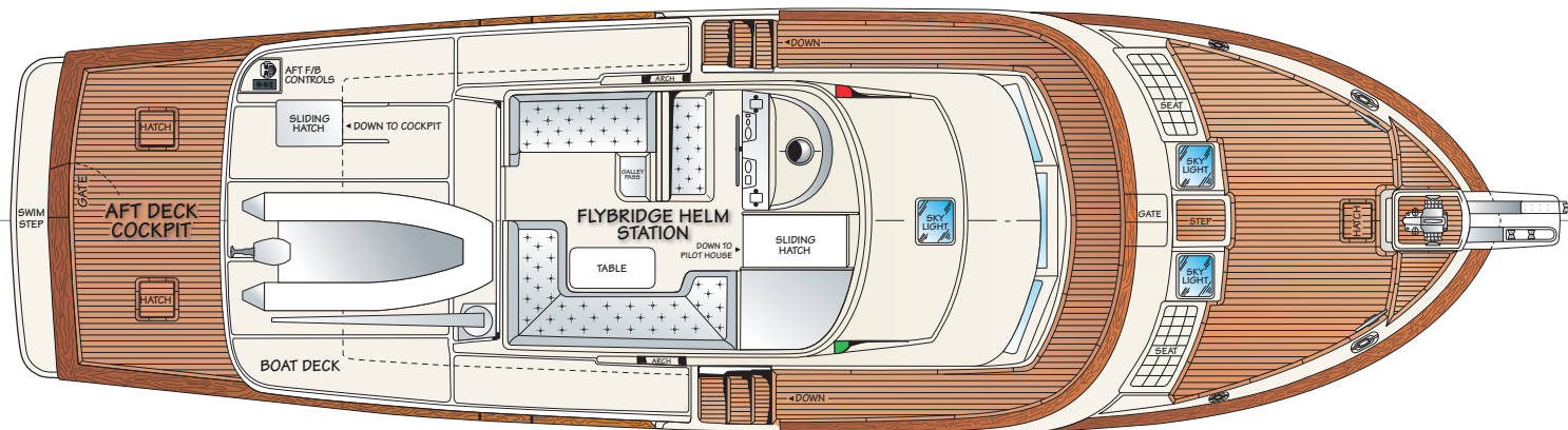
FLEMING 55' – FLYBRIDGE
